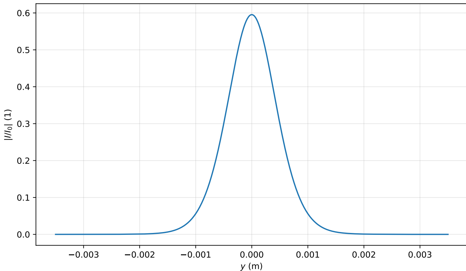
Intensity profile I(x=0, y, z=2.866)/I_0 , \text{Pin}=0.5\text{Pcr} , artificial time
